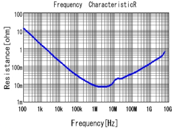
■ GRM155R61E225KE11 R DCOV, 25degC
