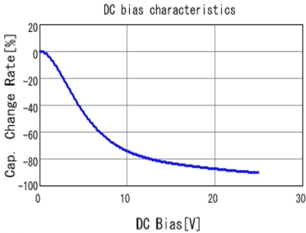
■ GRM155R61E225KE11 C-DC bias capchange, 25.0degC, AC1V
