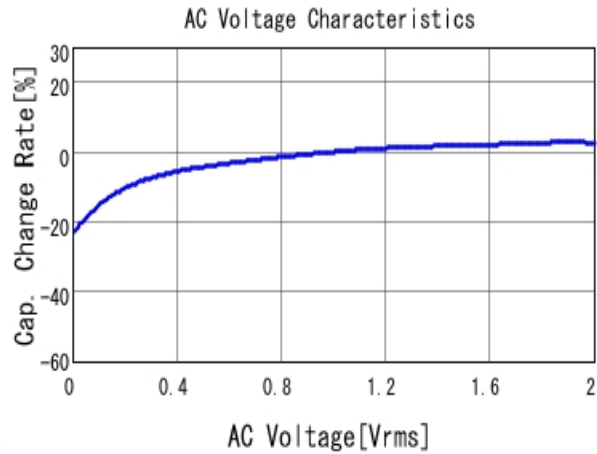
■ GRM155R61E225KE11 C-AC Voltage capchange, DCOV, 25.0d
