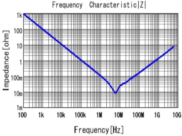
■ GRM155R61E225KE11 |Z| DCOV, 25degC
