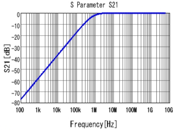
■ GRM155R61E222KA01 S21 DCOV, 25degC
