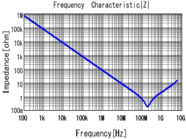
■ GRM155R61E222KA01 |Z| DCOV, 25degC
