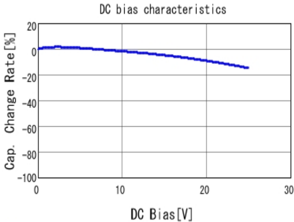
■ GRM155R61E222KA01 C-DC bias capchange, 25.0degC, AC1.
