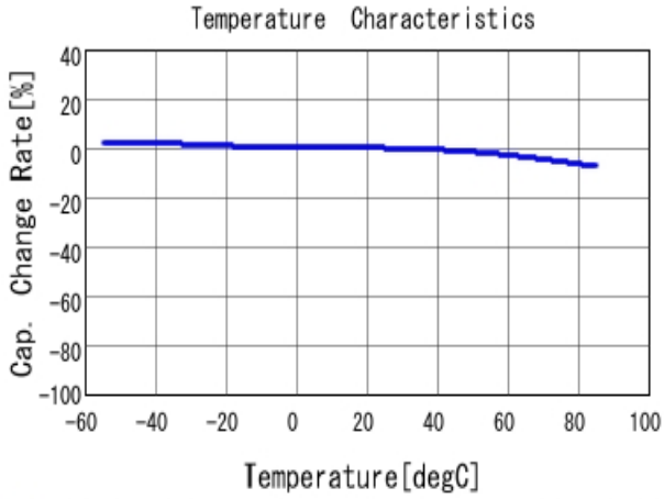
■ GRM155R61E222KA01 C-Temp. capchange, DCO. 0V, AC1.0V rm
