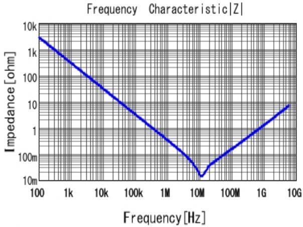
■ GRM155R61E105MA12 |Z| DCOV, 25degC
