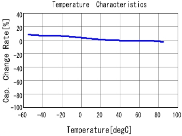
■ GRM155R61E105MA12 C-Temp. capchange, DC0.0V, AC1.0V r m
