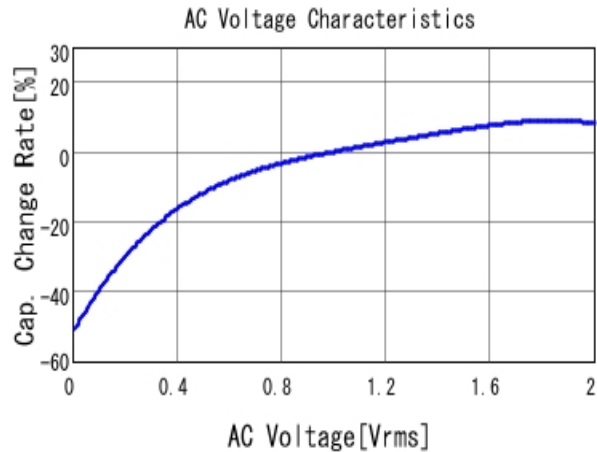
■ GRM155R61E105MA12 C-AC Voltage capchange, DCOV, 25.0d
