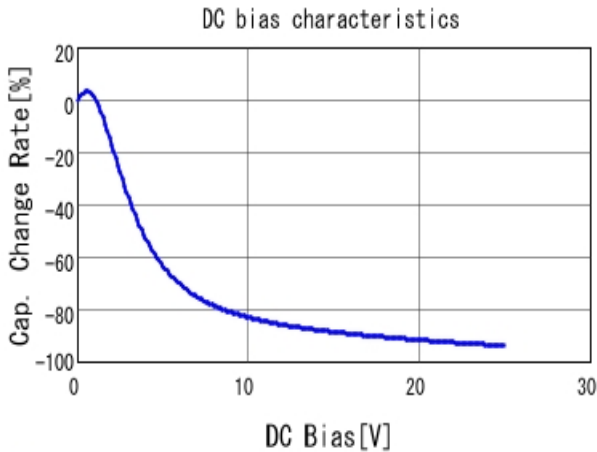
■ GRM155R61E105MA12 C-DC bias capchange, 25.0degC, AC1.
