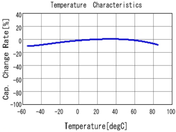
■ GRM155R61E105KE11 C-Temp. capchange, DCO. 0V, ACO. 5V rm
