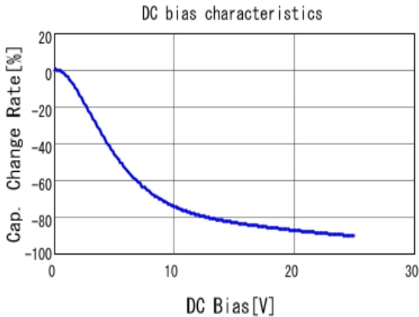
■ GRM155R61E105KE11 C-DC bias capchange, 25.0degC, AC1V
