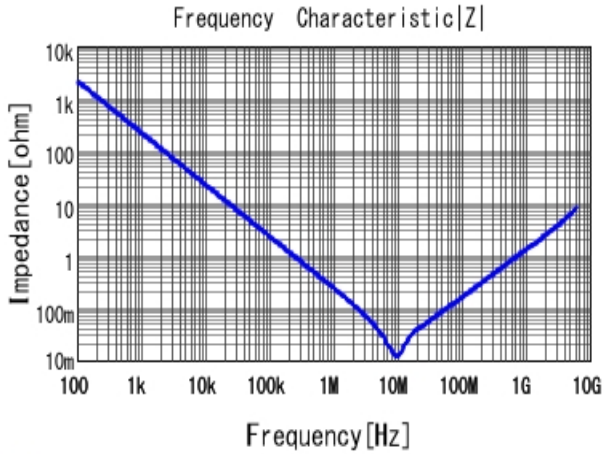
■ GRM155R61E105KE11 |Z| DCOV, 25degC
