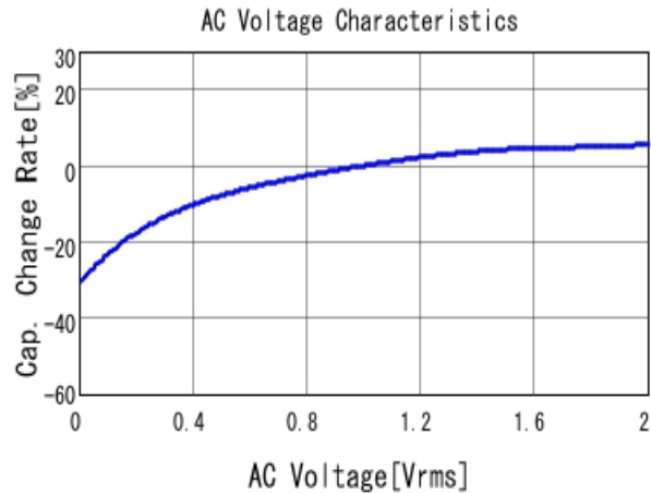
■ GRM155R61E105KE11 C-AC Voltage capchange, DCOV, 25.0d
