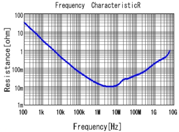
■ GRM155R61E105KE11 R DCOV, 25degC
