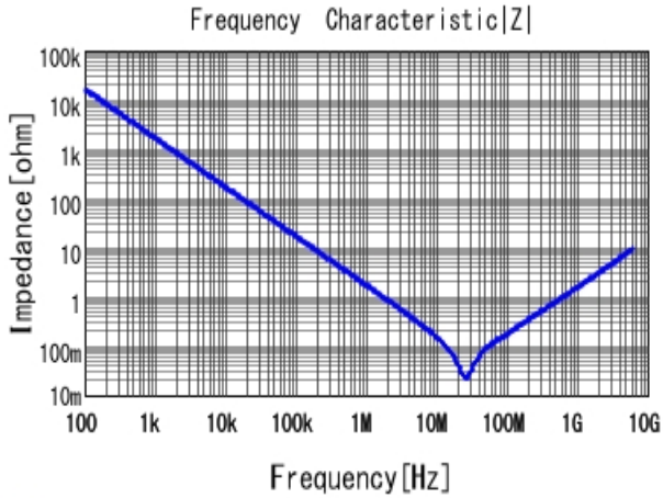
■ GRM155R61E104MA87 |Z| DCOV, 25degC
