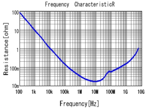
■ GRM155R61E104MA87 R DCOV, 25degC
