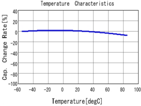
■ GRM155R61E104MA87 C-Temp. capchange, DC0.0V, AC1.0V rm
