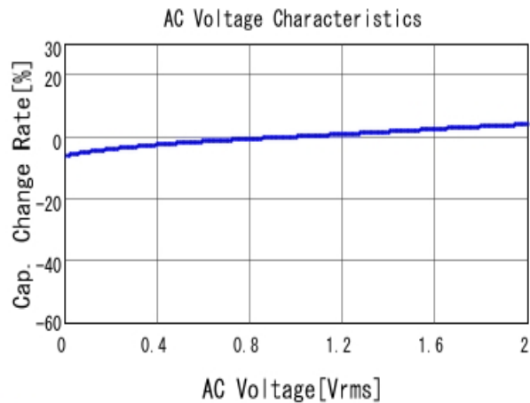
■ GRM155R61E104MA87 C-AC Voltage capchange, DCOV, 25.0d
