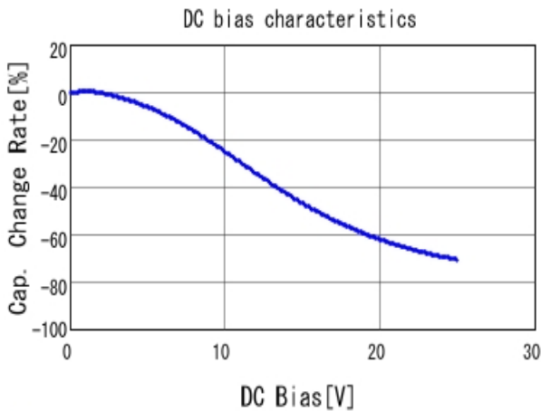
■ GRM155R61E104MA87 C-DC bias capchange, 25.0degC, AC1.
