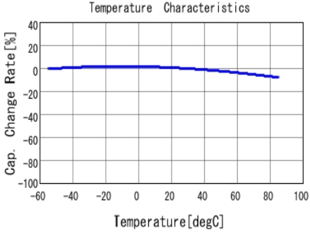
■ GRM155R61E104KA87 C-Temp. capchange, DC0.0V, AC1.0V r m
