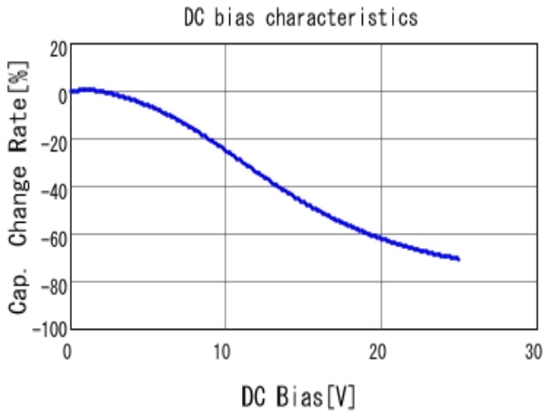
■ GRM155R61E104KA87 C-DC bias capchange, 25.0degC, AC1.
