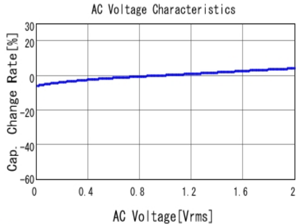
■ GRM155R61E104KA87 C-AC Voltage capchange, DCOV, 25.0d
