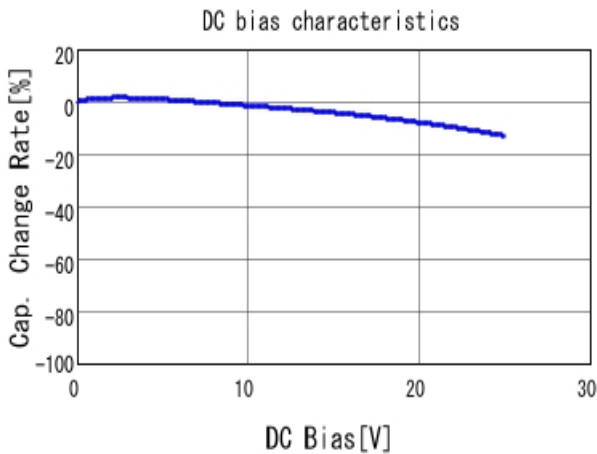
■ GRM155R61E102KA01 C-DC bias capchange, 25.0degC, AC1.
