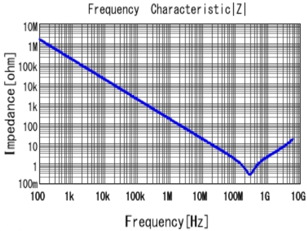
■ GRM155R61E102KA01 |Z| DCOV, 25degC
