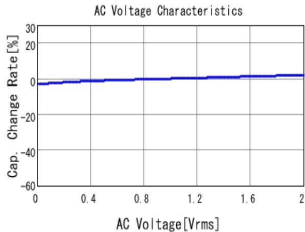
■ GRM155R61E102KA01 C-AC Voltage capchange, DCOV, 25.0d
