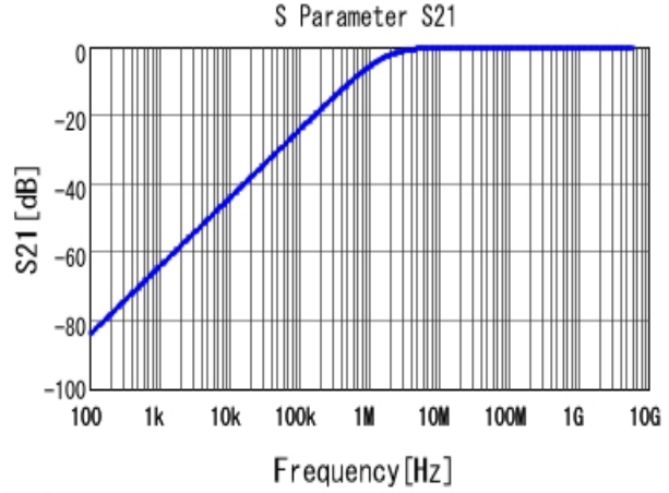
■ GRM155R61E102KA01 S21 DCOV, 25degC
