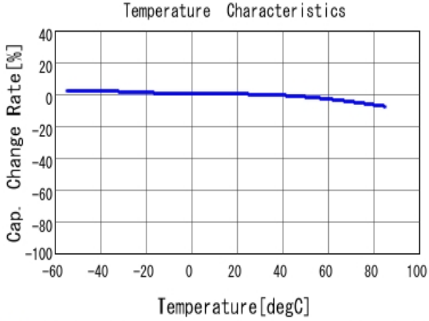
■ GRM155R61E102KA01 C-Temp. capchange, DCO. 0V, AC1.0V rm
