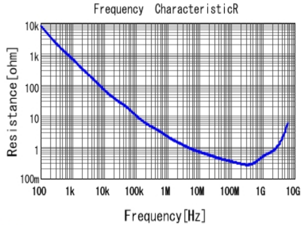
■ GRM155R61E102KA01 R DCOV, 25degC
