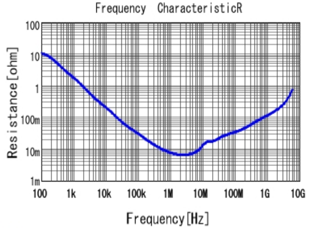
■ GRM155R61C225KE44 R DCOV, 25degC
