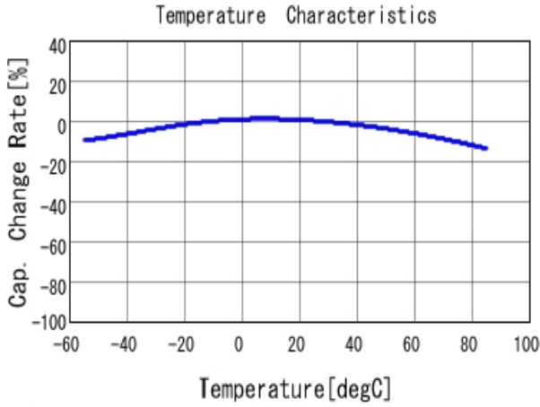
■ GRM155R61C225KE44 C-Temp. capchange, DC0.0V, AC0.2V rm
