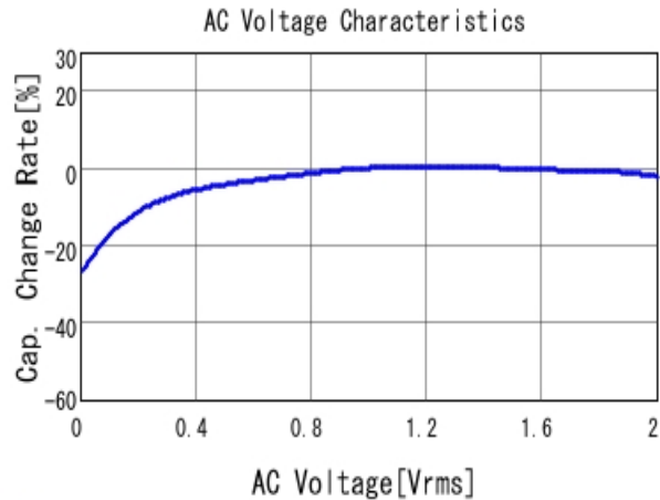
■ GRM155R61C225KE44 C-AC Voltage capchange, DCOV, 25.0d
