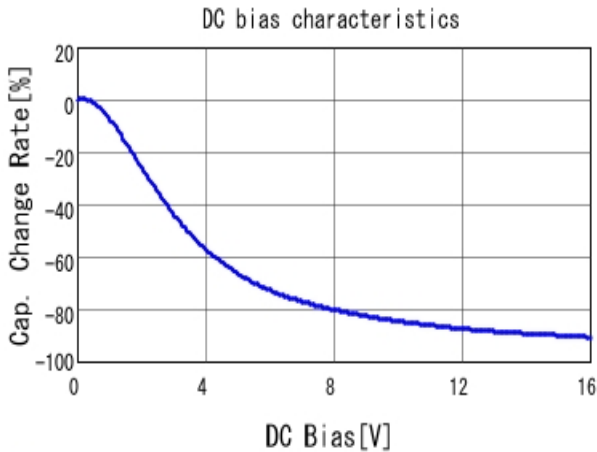
■ GRM155R61C225KE44 C-DC bias capchange, 25.0degC, AC1V
