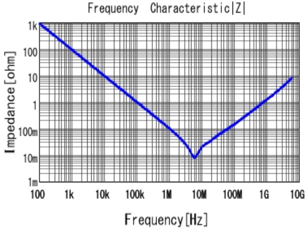
■ GRM155R61C225KE44 |Z| DCOV, 25degC
