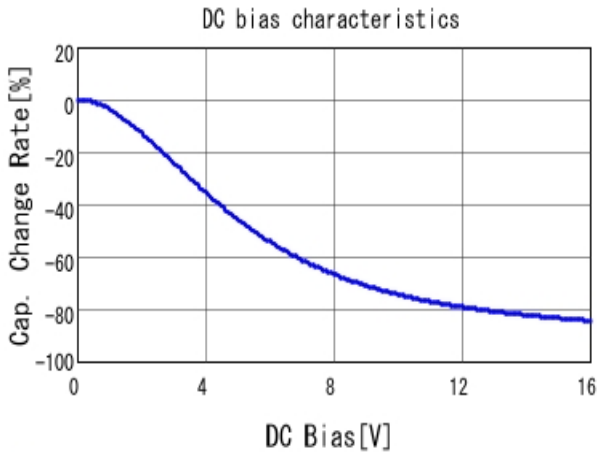
■ GRM155R61C225KE11 C-DC bias capchange, 25.0degC, AC1V
