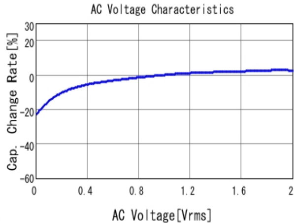
■ GRM155R61C225KE11 C-AC Voltage capchange, DCOV, 25.0d
