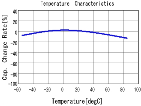
■ GRM155R61C225KE11 C-Temp. capchange, DCO. 0V, ACO. 2V rm
