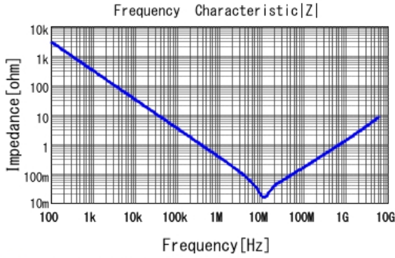
■ GRM155R61C105MA12 |Z| DCOV, 25degC
