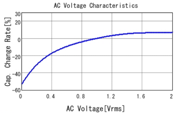
■ GRM155R61C105MA12 C-AC Voltage capchange, DCOV, 25.0d
