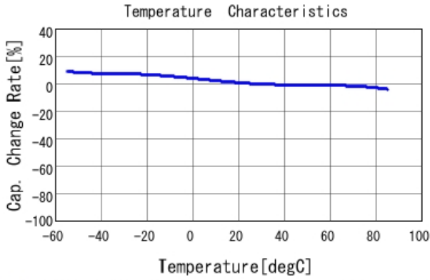
■ GRM155R61C105KA12 C-Temp. capchange, DCO. 0V, AC1. 0Vrm
