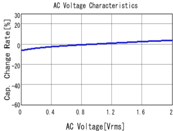
■ GRM155R61C104KA88 C-AC Voltage capchange, DCOV, 25.0d
