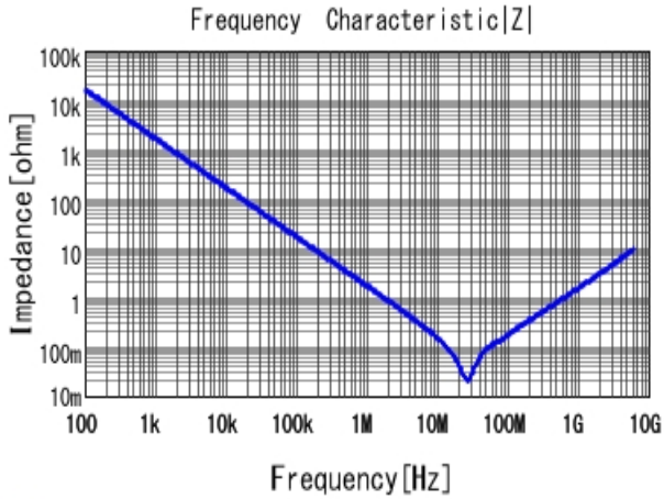
■ GRM155R61C104KA88 |Z| DCOV, 25degC
