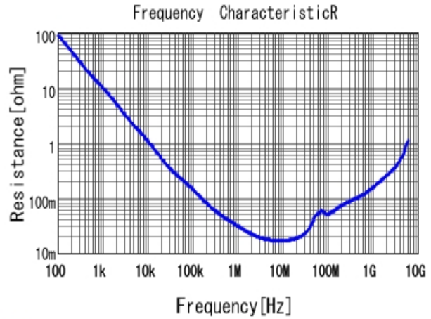
■ GRM155R61C104KA88 R DCOV, 25degC
