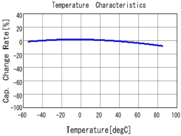
■ GRM155R61C104KA88 C-Temp. capchange, DC0.0V, AC1.0V r m
