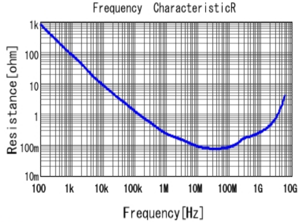
■ GRM155R61C103KA01 R DCOV, 25degC
