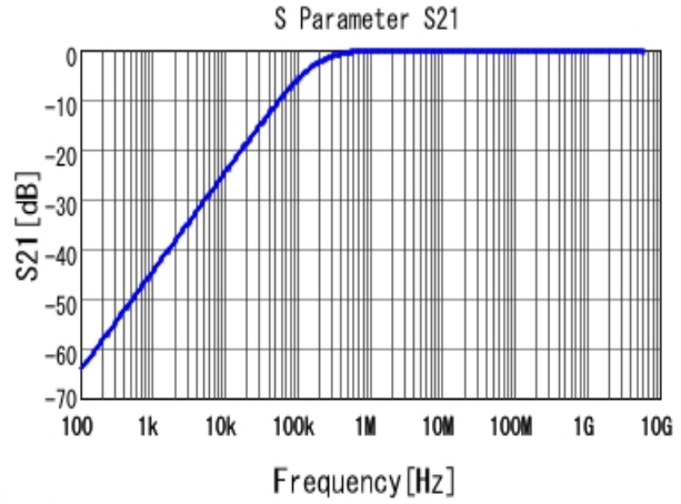
■ GRM155R61C103KA01 S21 DCOV, 25degC
