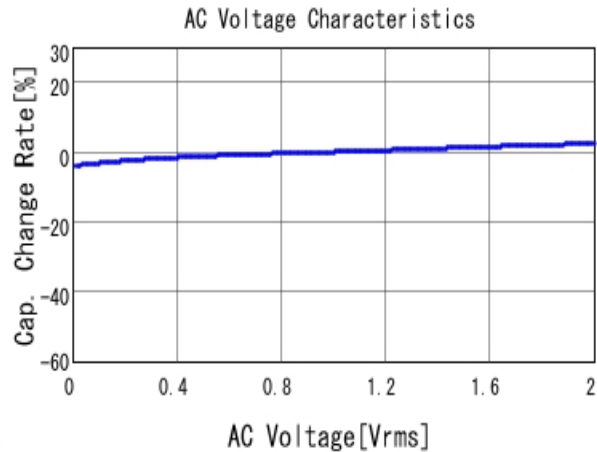
■ GRM155R61C103KA01 C-AC Voltage capchange, DCOV, 25.0d
