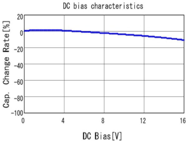
■ GRM155R61C103KA01 C-DC bias capchange, 25.0degC, AC1.
