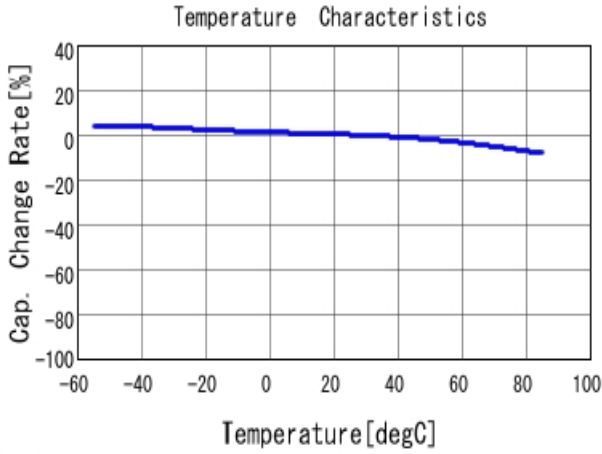
■ GRM155R61C103KA01 C-Temp. capchange, DCO. 0V, AC1.0V rm
