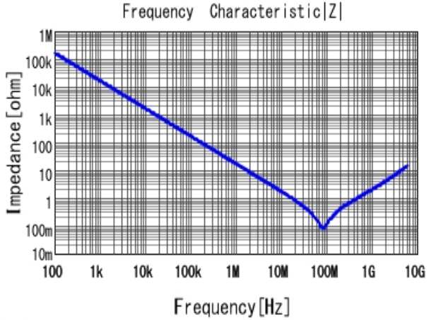
■ GRM155R61C103KA01 |Z| DCOV, 25degC
