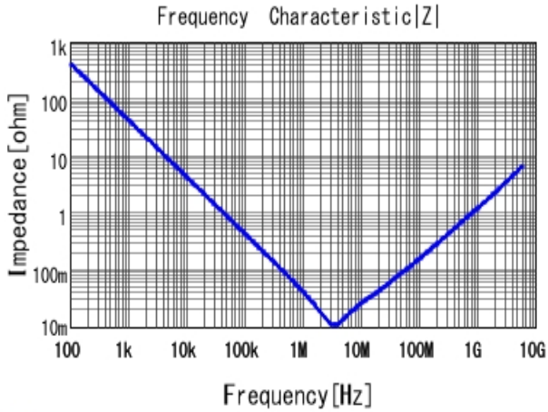
■ GRM155R61A475MEAA |Z| DCOV, 25degC
