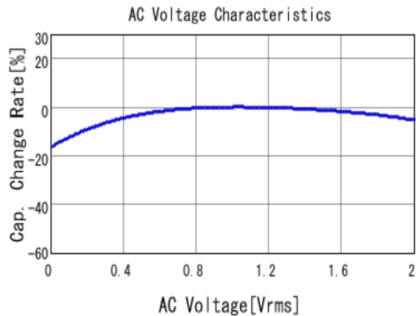
■ GRM155R61A475MEAA C-AC Voltage capchange, DCOV, 25.0d
