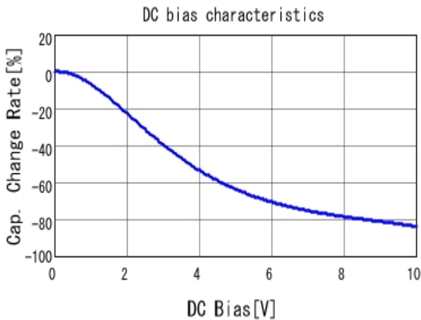
■ GRM155R61A475MEAA C-DC bias capchange, 25.0degC, AC1V
