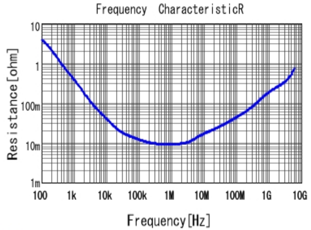
■ GRM155R61A475MEAA R DCOV, 25degC
