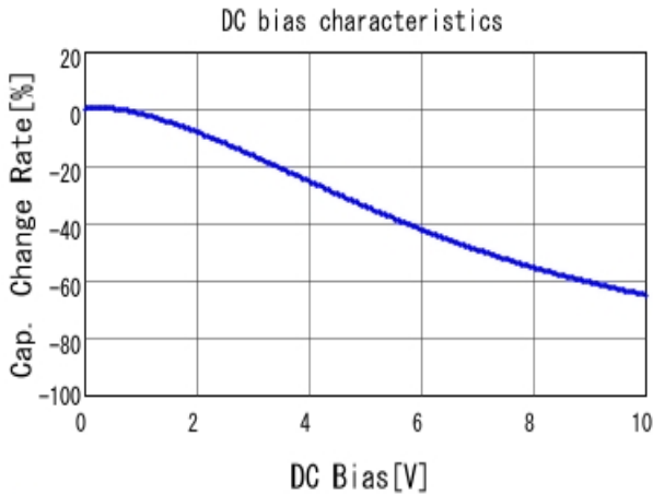
■ GRM155R61A474KE15 C-DC bias capchange, 25.0degC, AC0.
