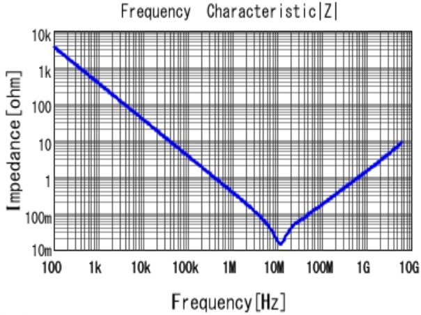
■ GRM155R61A474KE15 |Z| DCOV, 25degC
