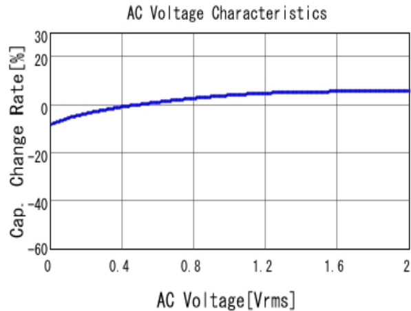
■ GRM155R61A474KE15 C-AC Voltage capchange, DCOV, 25.0d
