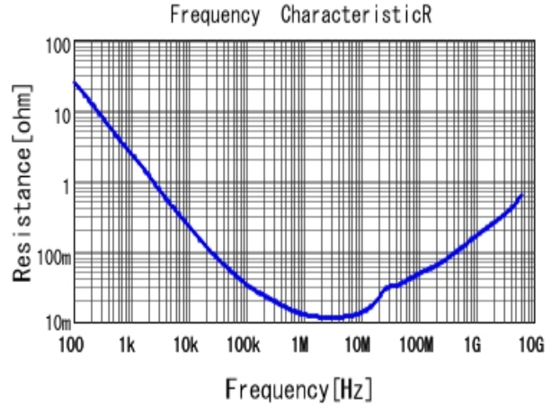
■ GRM155R61A474KE15 R DCOV, 25degC
