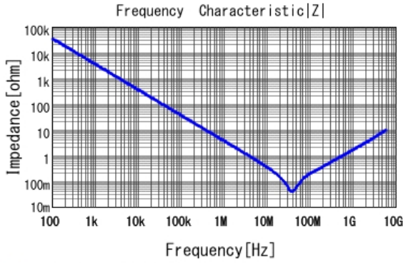
■ GRM155R61A473KA01 |Z| DCOV, 25degC
