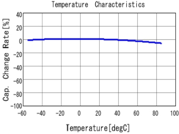
■ GRM155R61A333KA01 C-Temp. capchange, DCO. 0V, AC1.0V rm
