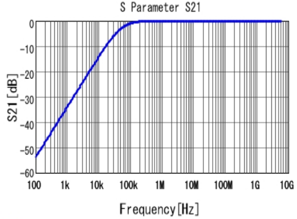
■ GRM155R61A333KA01 S21 DCOV, 25degC
