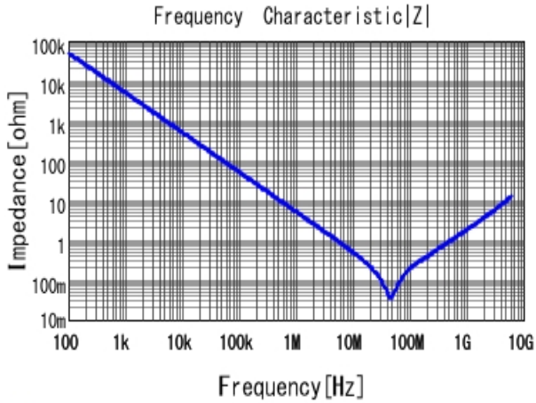
■ GRM155R61A333KA01 |Z| DCOV, 25degC
