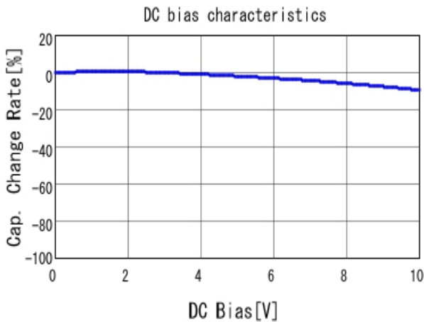
■ GRM155R61A333KA01 C-DC bias capchange, 25.0degC, AC1.
