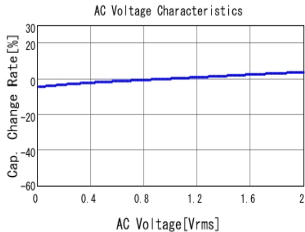
■ GRM155R61A333KA01 C-AC Voltage capchange, DCOV, 25.0d
