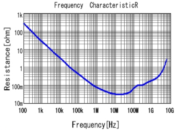
■ GRM155R61A333KA01 R DCOV, 25degC
