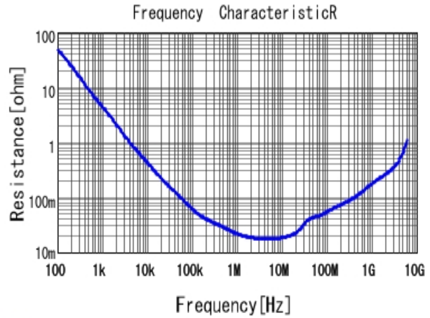
■ GRM155R61A224KE19 R DCOV, 25degC
