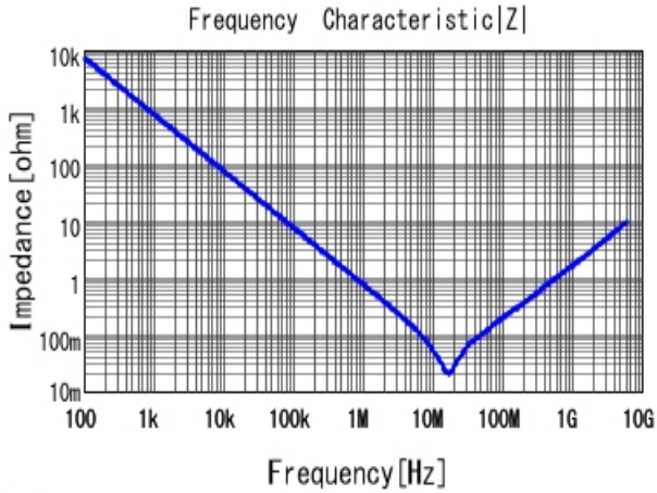
■ GRM155R61A224KE19 |Z| DCOV, 25degC
