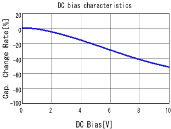
■ GRM155R61A224KE19 C-DC bias capchange, 25.0degC, AC0.
