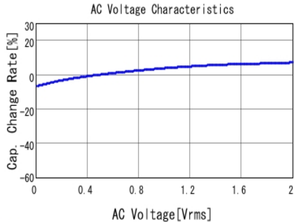
■ GRM155R61A224KE19 C-AC Voltage capchange, DCOV, 25.0d
