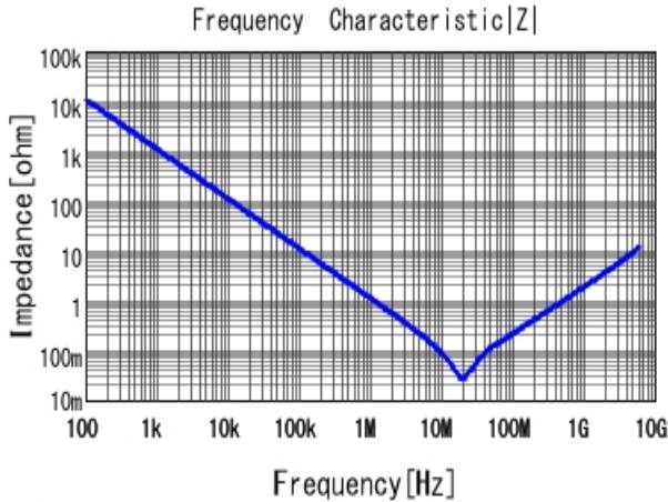
■ GRM155R61A154KE19 |Z| DC0V, 25degC
