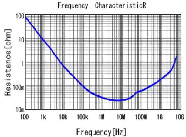
■ GRM155R61A154KE19 R DC0V, 25degC
