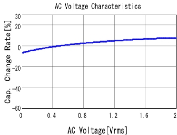
■ GRM155R61A154KE19 C-AC Voltage capchange, DC0V, 25.0d
