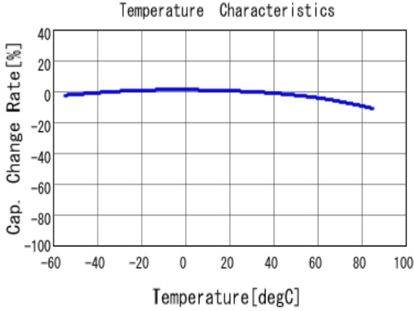
■ GRM155R61A105KE15 C-Temp. capchange, DCO. 0V, ACO. 5V rm
