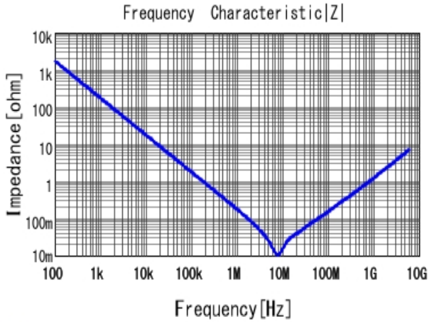
■ GRM155R61A105KE15 |Z| DCOV, 25degC
