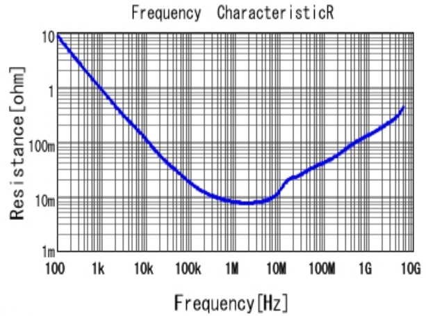
■ GRM155R61A105KE15 R DCOV, 25degC
