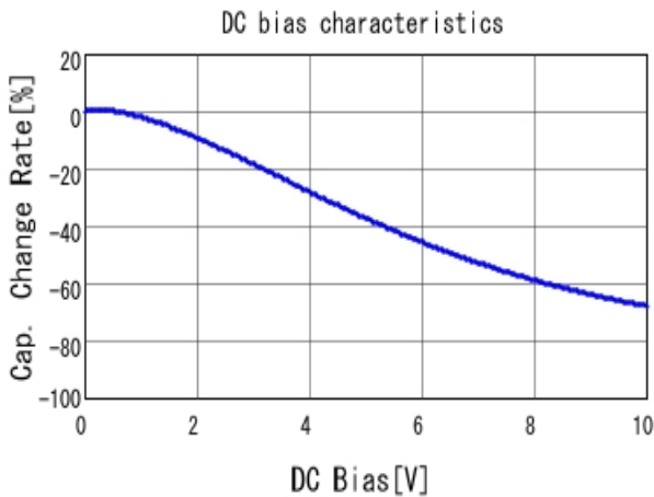
■ GRM155R61A105KE15 C-DC bias capchange, 25.0degC, AC0.
