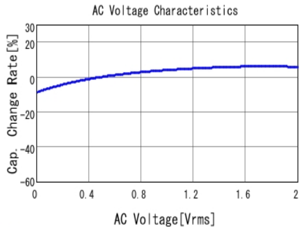
■ GRM155R61A105KE15 C-AC Voltage capchange, DCOV, 25.0d
