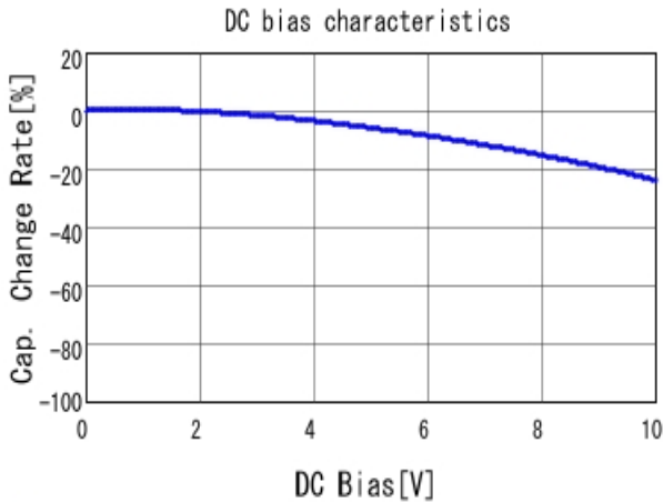
■ GRM155R61A104KA01 C-DC bias capchange, 25.0degC, AC1.
