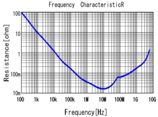
■ GRM155R61A104KA01 R DCOV, 25degC
