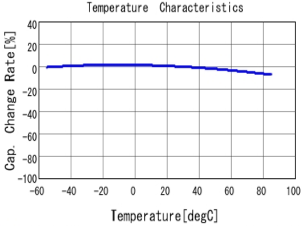
■ GRM155R61A104KA01 C-Temp. capchange, DC0.0V, AC1.0V rm
