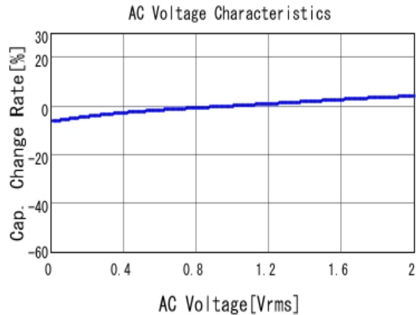
■ GRM155R61A104KA01 C-AC Voltage capchange, DCOV, 25.0d
