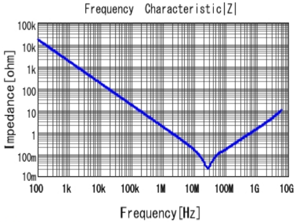
■ GRM155R61A104KA01 |Z| DCOV, 25degC
