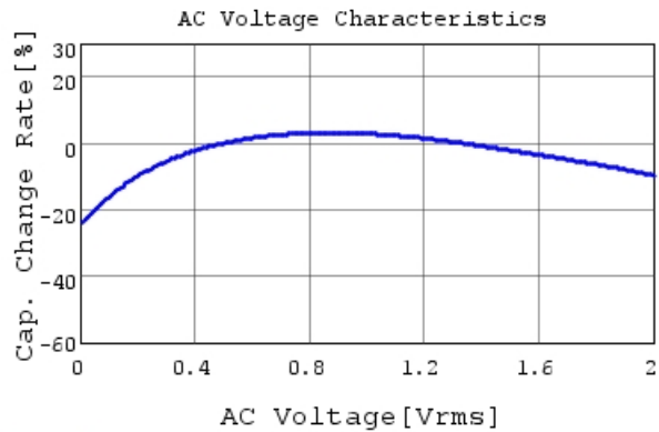
GRM155R60J475ME87 C-AC Voltage capchange, DC
