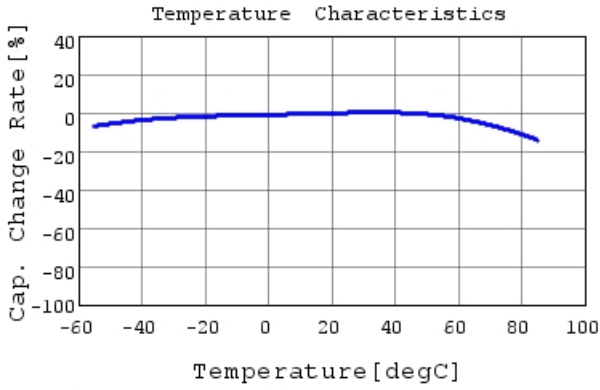
GRM155R60J475ME87 C-Temp. capchange, DC0.0V,
