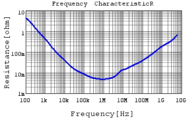
GRM155R60J475ME87 R DC0V, 25degC
