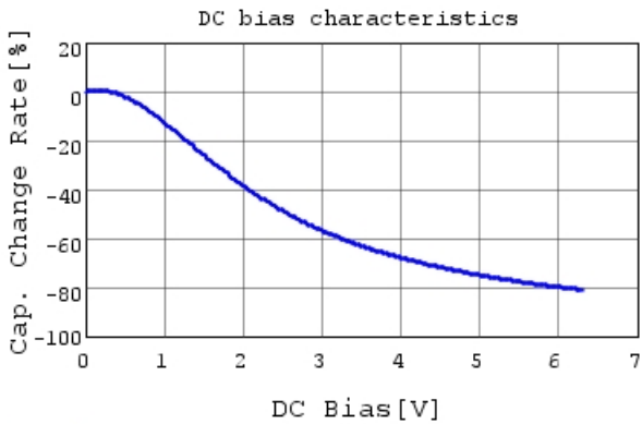
GRM155R60J475ME87 C-DC bias capchange, 25.0c
