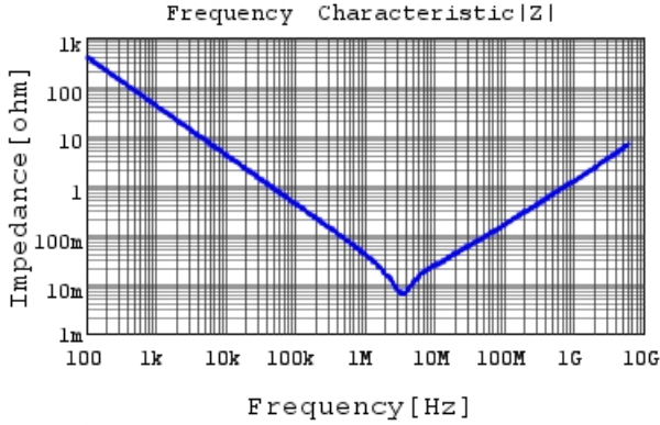
GRM155R60J475ME87 |Z| DC0V, 25degC
