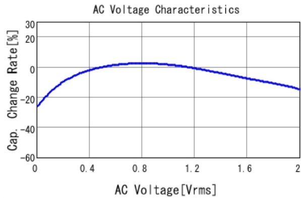
GRM155R60J475ME47 C-AC Voltage capchange, DCOV, 25
