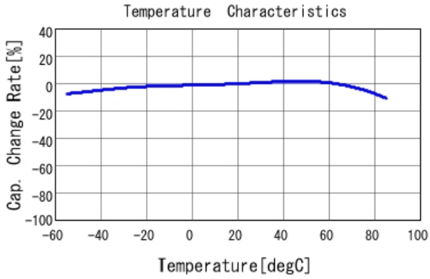
GRM155R60J475ME47 C-Temp. capchange, DC0.0V, AC0.2
