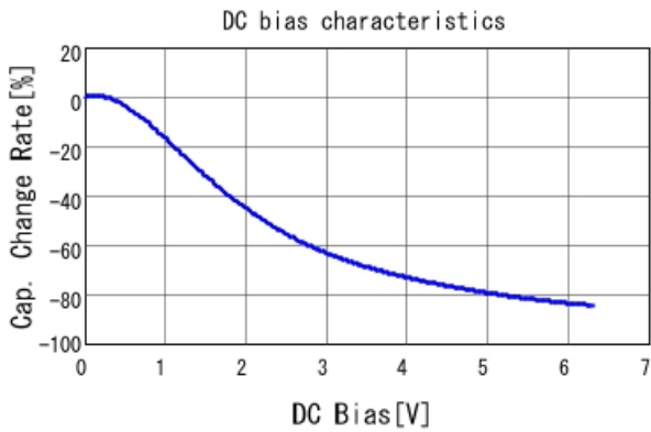
GRM155R60J475ME47 C-DC bias capchange, 25.0degC, A
