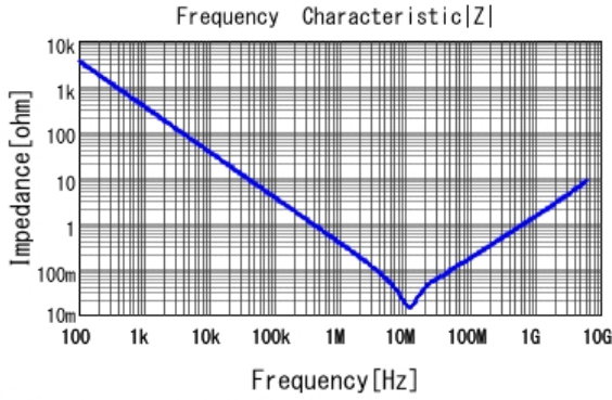
■ GRM155R60J474KE19 |Z| DCOV, 25degC
