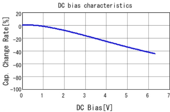
■ GRM155R60J474KE19 C-DC bias capchange, 25.0degC, AC0.
