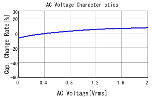
■ GRM155R60J224KE01 C-AC Voltage capchange, DCOV, 25.0d
