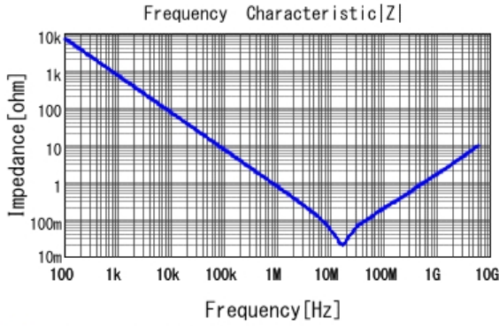
■ GRM155R60J224KE01 |Z| DCOV, 25degC
