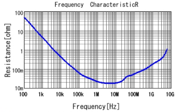
■ GRM155R60J224KE01 R DCOV, 25degC
