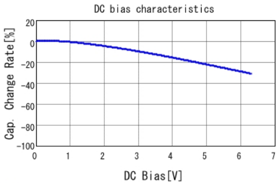
■ GRM155R60J224KE01 C-DC bias capchange, 25.0degC, AC0.
