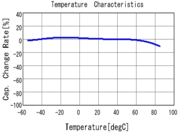
■ GRM155R60J105KE19 C-Temp. capchange, DC0.0V, AC0.5V rm
