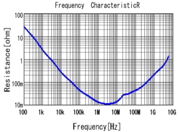
■ GRM155R60J105KE19 R DCOV, 25degC
