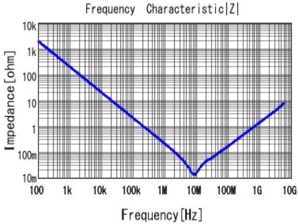
■ GRM155R60J105KE19 |Z| DCOV, 25degC
