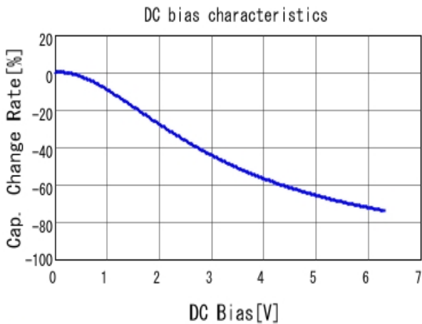
■ GRM155R60J105KE19 C-DC bias capchange, 25.0degC, AC0.
