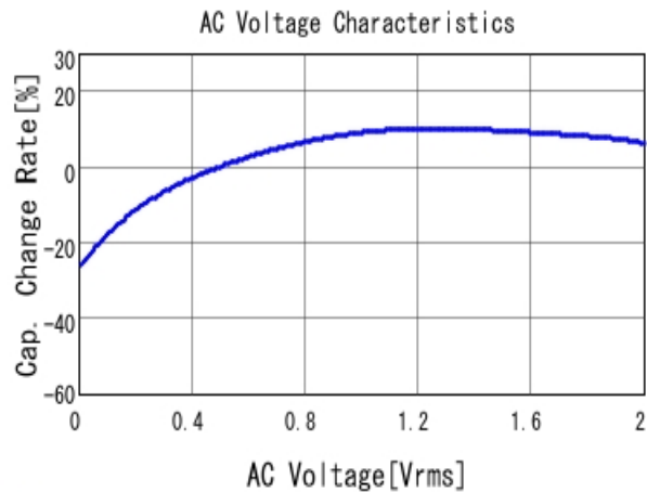
■ GRM155R60J105KE19 C-AC Voltage capchange, DCOV, 25.0d
