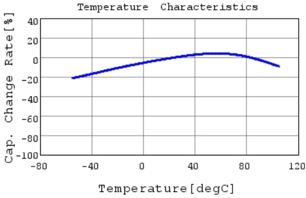
GRM155C81E105KE11 C-Temp. capchange, DC0.0V,
