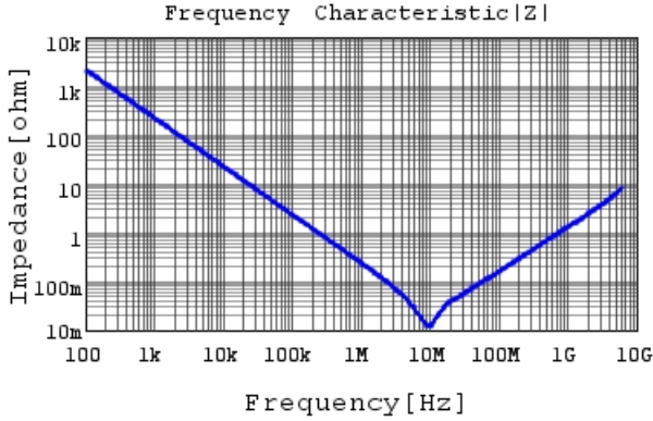
GRM155C81E105KE11 |Z| DCOV, 25degC
