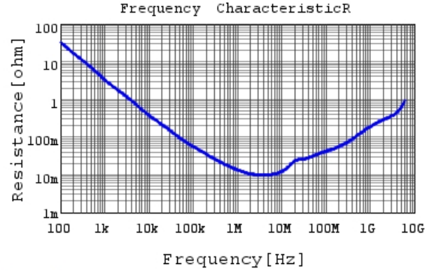
GRM155C81E105KE11 R DCOV, 25degC
