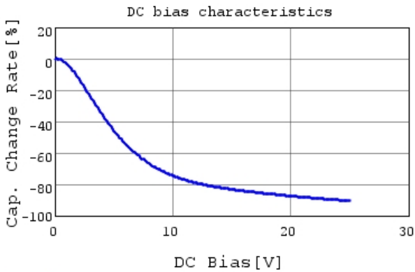
GRM155C81E105KE11 C-DC bias capchange, 25.0c
