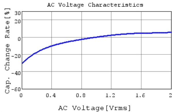
GRM155C81E105KE11 C-AC Voltage capchange, Dc
