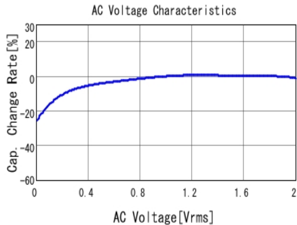
■ GRM155C81A225KE44 C-AC Voltage capchange, DCOV, 25.0d
