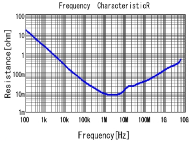
■ GRM155C81A225KE44 R DCOV, 25degC
