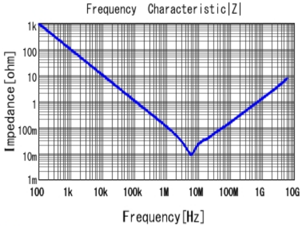
■ GRM155C81A225KE44 |Z| DCOV, 25degC
