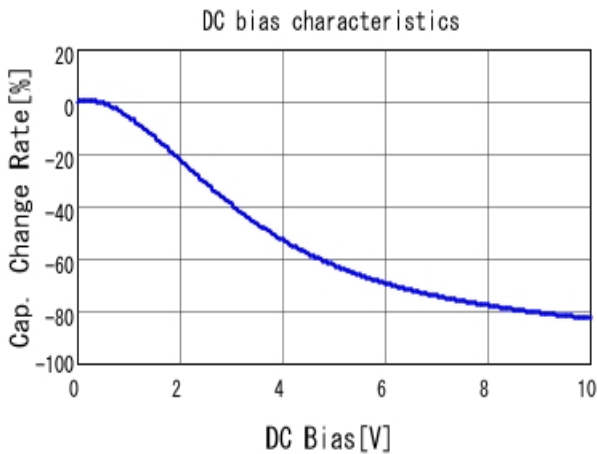
■ GRM155C81A225KE44 C-DC bias capchange, 25.0degC, AC1V
