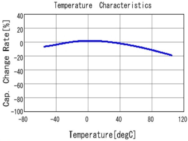
■ GRM155C81A225KE44 C-Temp. capchange, DCO. 0V, ACO. 2V rm
