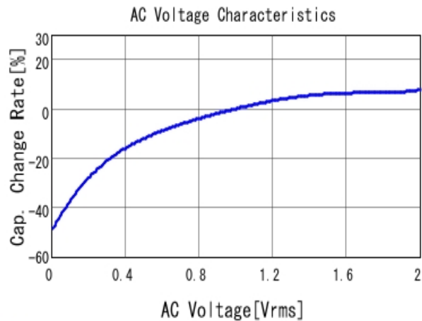
■ GRM155C81A105KA12 C-AC Voltage capchange, DCOV, 25.0d
