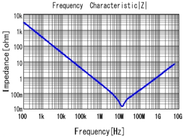
■ GRM155C81A105KA12 |Z| DCOV, 25degC
