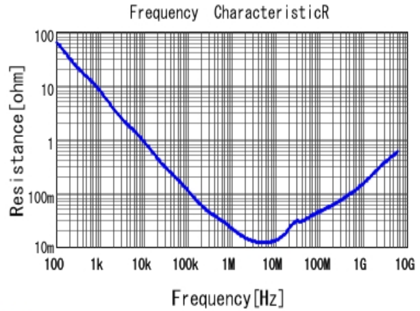
■ GRM155C81A105KA12 R DCOV, 25degC
