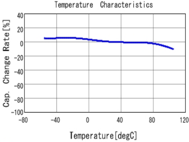
■ GRM155C81A105KA12 C-Temp. capchange, DC0.0V, AC1.0V rm
