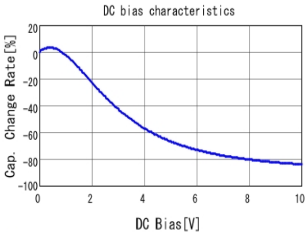
■ GRM155C81A105KA12 C-DC bias capchange, 25.0degC, AC1.
