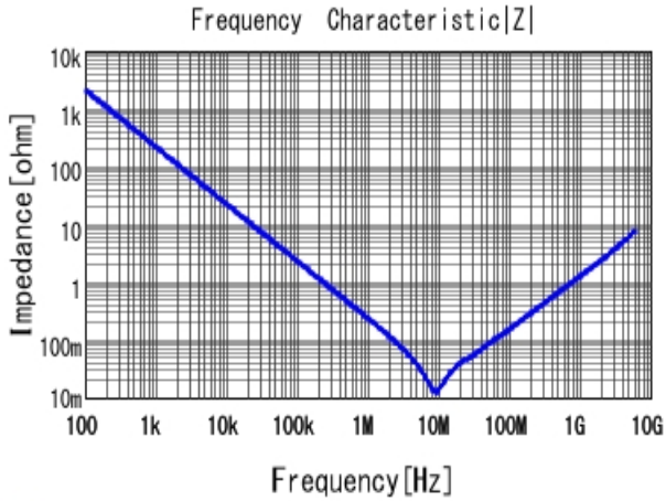
■ GRM155C71A105KE11 |Z| DCOV, 25degC
