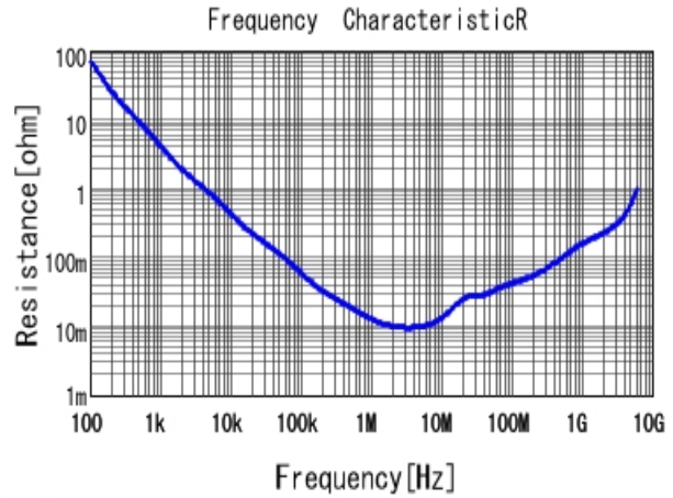
■ GRM155C71A105KE11 R DCOV, 25degC
