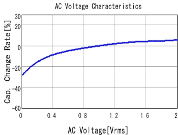
■ GRM155C71A105KE11 C-AC Voltage capchange, DCOV, 25.0d
