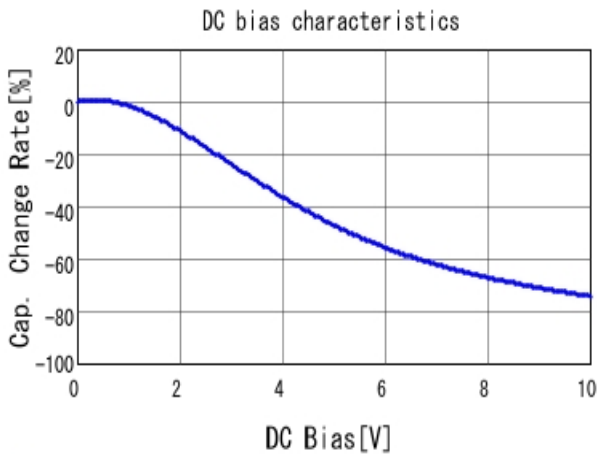
■ GRM155C71A105KE11 C-DC bias capchange, 25.0degC, AC1V
