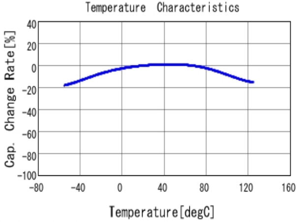
■ GRM155C71A105KE11 C-Temp. capchange, DCO. 0V, ACO. 2V rm
