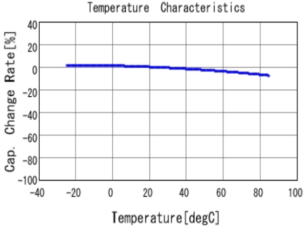
■ GRM155B31H104KE14 C-Temp. capchange, DC0.0V, AC1.0V rm
