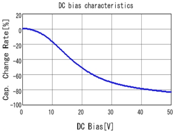
■ GRM155B31H104KE14 C-DC bias capchange, 20.0degC, AC1.
