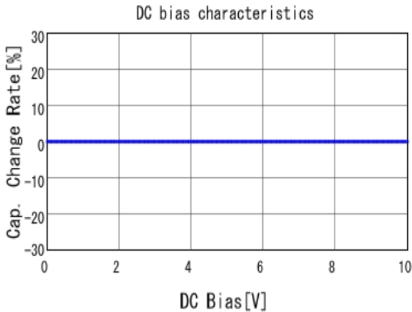
■ GRM1557U1A272JA01 C-DC bias capchange, 25.0degC, AC1V
