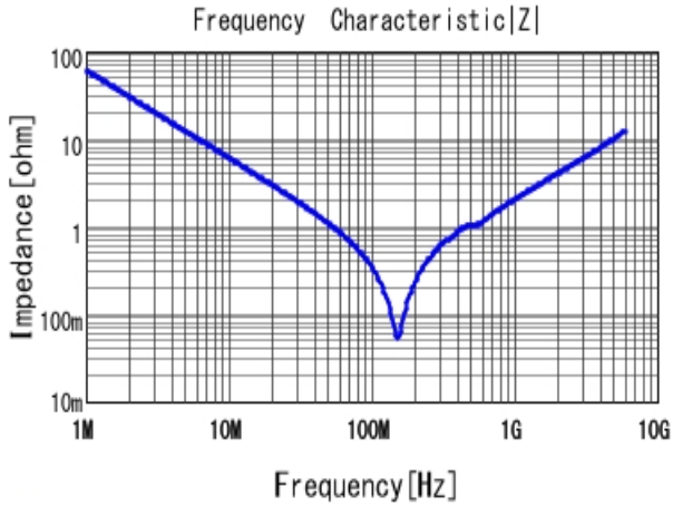
■ GRM1557U1A272JA01 |Z| DCOV, 25degC
