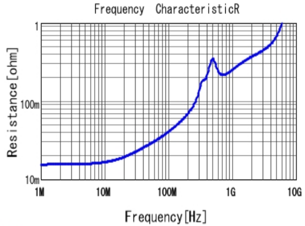
■ GRM1557U1A272JA01 R DCOV, 25degC
