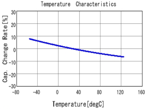
■ GRM1557U1A272JA01 C-Temp. capchange, DCOV, AC1Vrms
