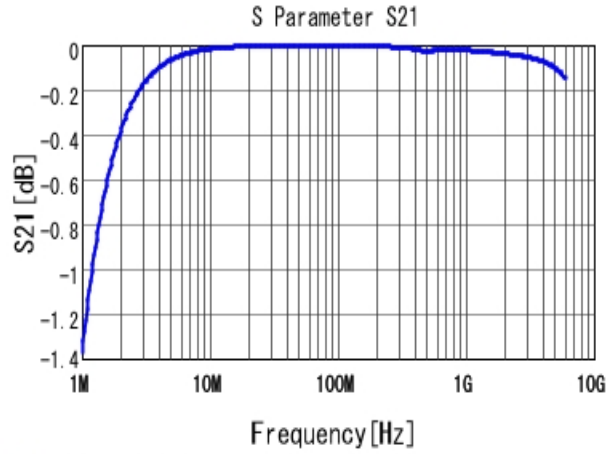
■ GRM1557U1A272JA01 S21 DCOV, 25degC
