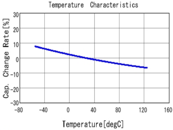
■ GRM1557U1A182JA01 C-Temp. capchange, DCOV, AC1Vrms
