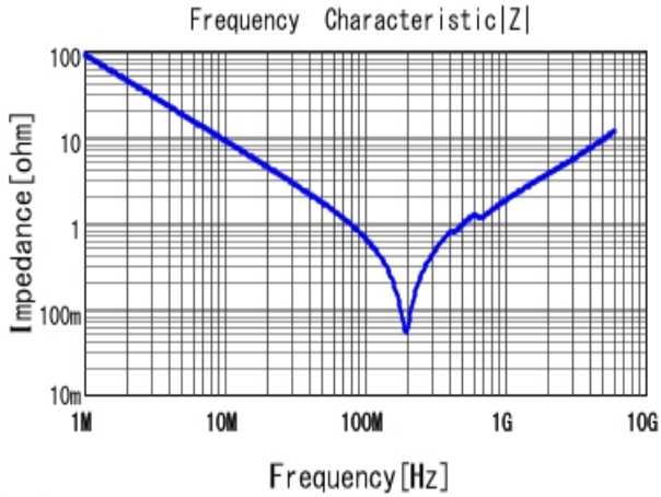
■ GRM1557U1A182JA01 |Z| DCOV, 25degC
