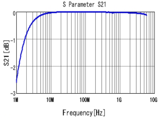
■ GRM1557U1A182JA01 S21 DCOV, 25degC
