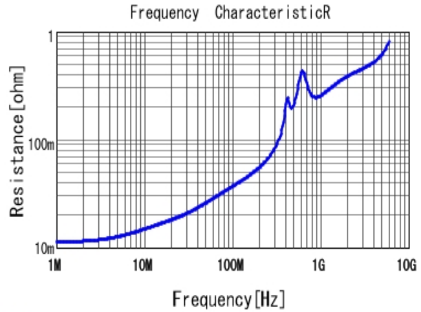
■ GRM1557U1A182JA01 R DCOV, 25degC
