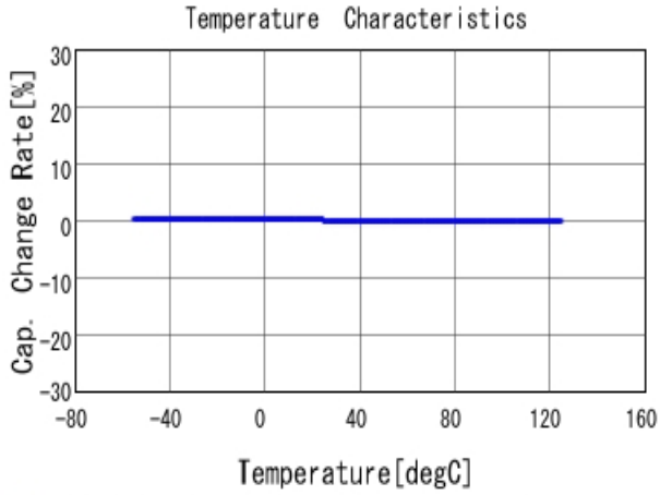
■ GRM1555C2A470JA01 C-Temp. capchange, DCOV, AC1Vrms
