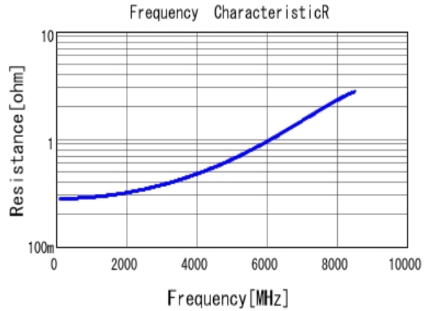
■ GRM1555C2A3R0CA01 R DC0V, 25degC
