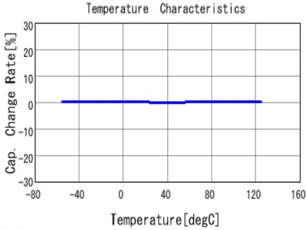
■ GRM1555C2A3R0CA01 C-Temp. capchange, DCOV, AC1Vrms
