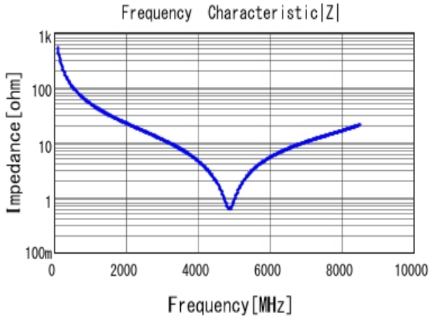
■ GRM1555C2A3R0CA01 |Z| DC0V, 25degC
