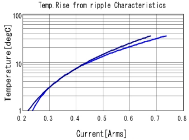
GRM1555C2A3R0CA01 Temp. rise ■ 2GHz ■ 3GHz
