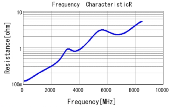
■ GRM1555C2A330JA01 R DCOV, 25degC
