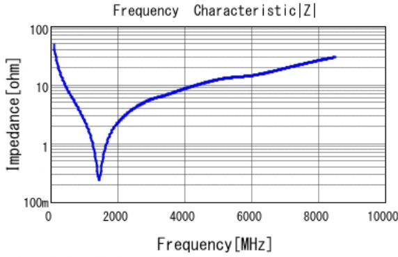
■ GRM1555C2A330JA01 |Z| DCOV, 25degC
