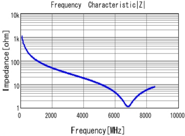
■ GRM1555C2A1R5CA01 |Z| DCOV, 25degC
