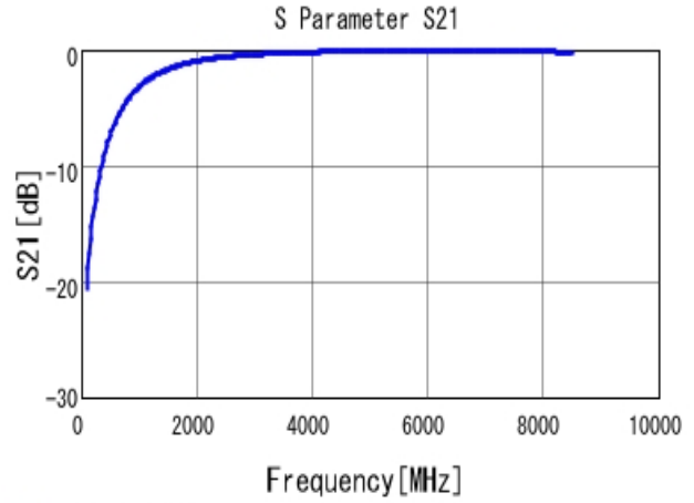
■ GRM1555C2A1R5CA01 S21 DCOV, 25degC
