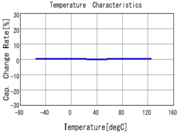
■ GRM1555C2A1R5CA01 C-Temp. capchange, DCOV, AC1Vrms
