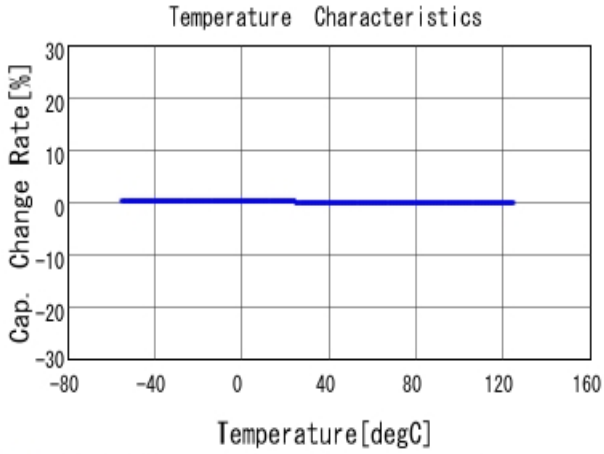
■ GRM1555C2A101JA01 C-Temp. capchange, DCOV, AC1Vrms
