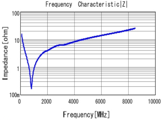
■ GRM1555C2A101JA01 |Z| DCOV, 25degC
