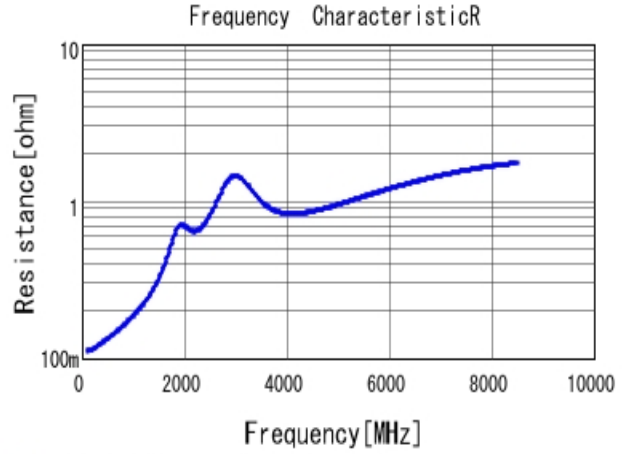
■ GRM1555C2A101JA01 R DCOV, 25degC
