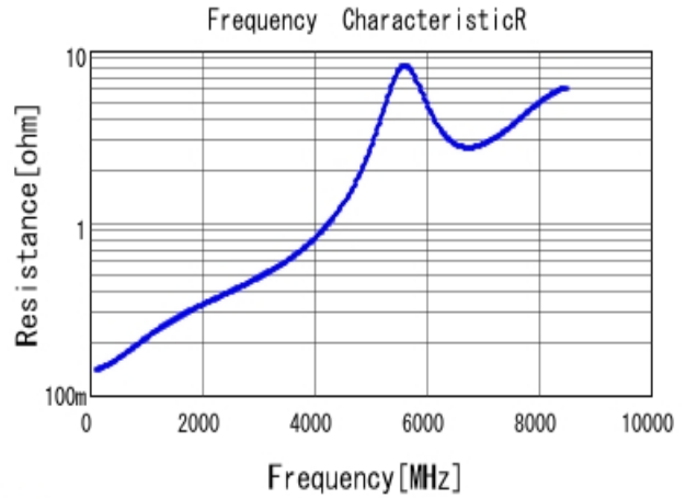
■ GRM1555C2A100JA01 R DCOV, 25degC
