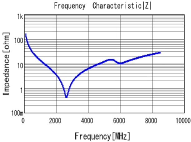
■ GRM1555C2A100JA01 |Z| DCOV, 25degC
