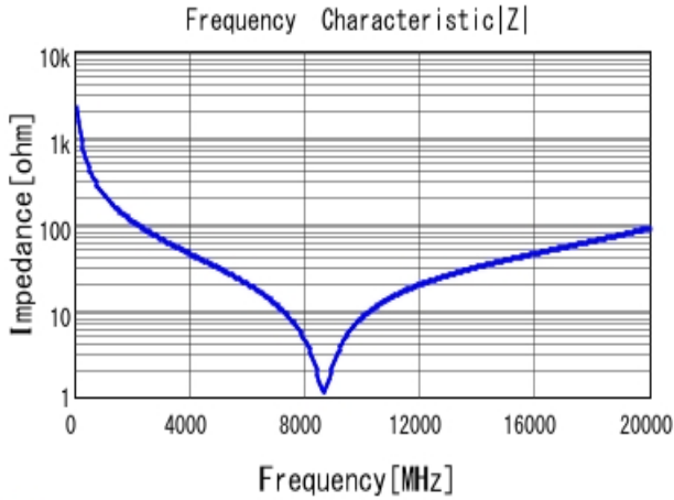
■ GRM1555C1HR70BA01 |Z| DCOV, 25degC
