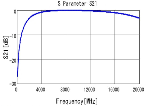
■ GRM1555C1HR70BA01 S21 DCOV, 25degC
