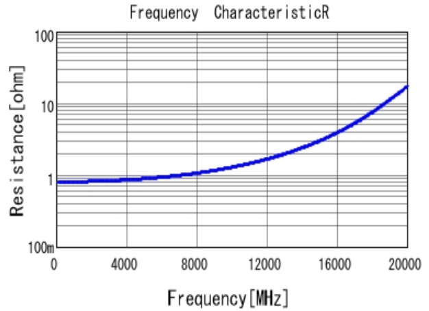
■ GRM1555C1HR70BA01 R DCOV, 25degC
