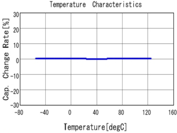
■ GRM1555C1HR70BA01 C-Temp. capchange, DCOV, AC1Vrms
