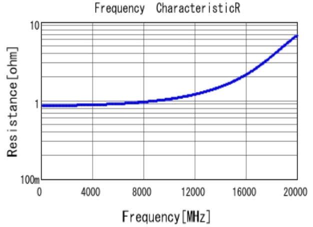
■ GRM1555C1HR50BA01 R DCOV, 25degC
