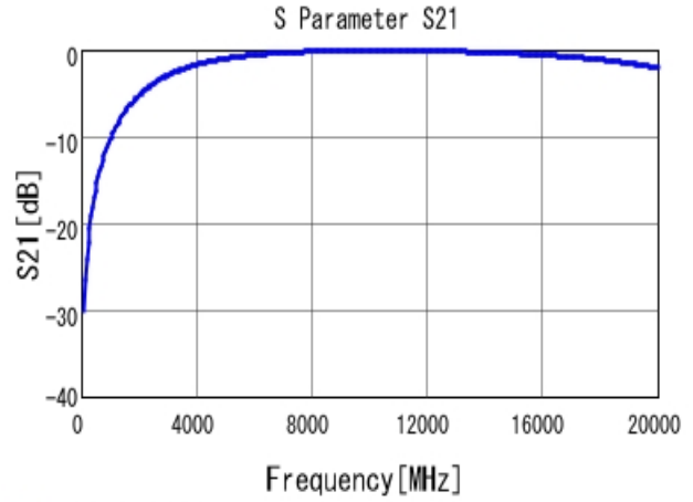
■ GRM1555C1HR50BA01 S21 DCOV, 25degC
