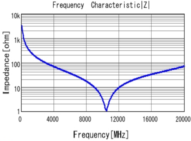
■ GRM1555C1HR50BA01 |Z| DCOV, 25degC
