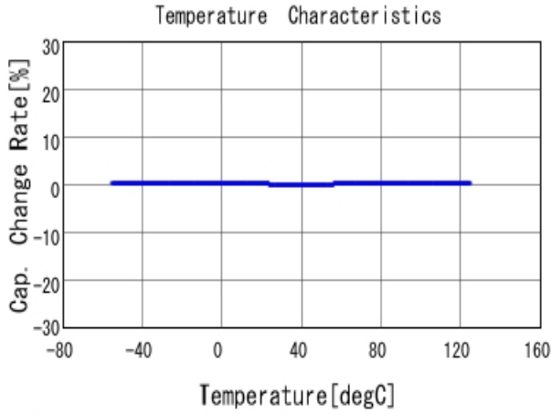
■ GRM1555C1HR50BA01 C-Temp. capchange, DCOV, AC1Vrms
