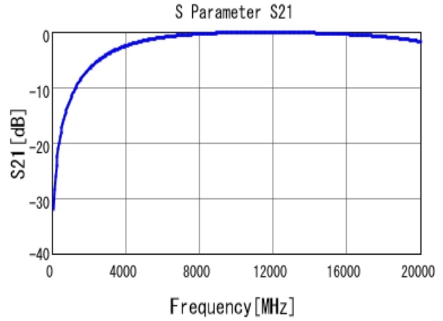
■ GRM1555C1HR40BA01 S21 DCOV, 25degC
