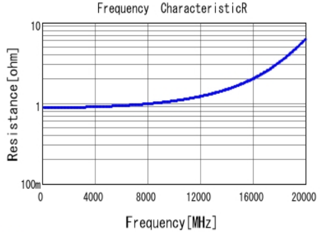
■ GRM1555C1HR40BA01 R DCOV, 25degC
