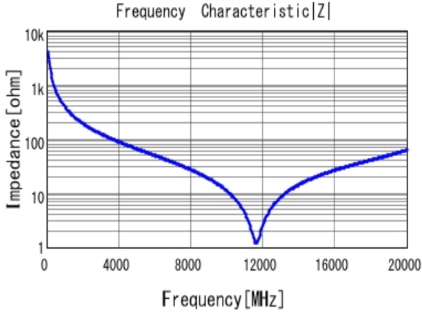
■ GRM1555C1HR40BA01 |Z| DCOV, 25degC
