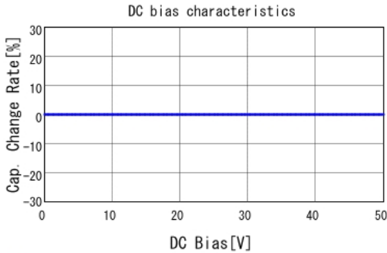
■ GRM1555C1HR30BA01 C-DC bias capchange, 25.0degC, AC1V
