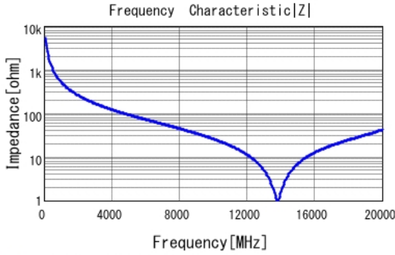
■ GRM1555C1HR30BA01 |Z| DCOV, 25degC
