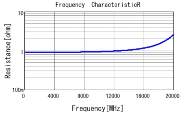
■ GRM1555C1HR30BA01 R DCOV, 25degC
