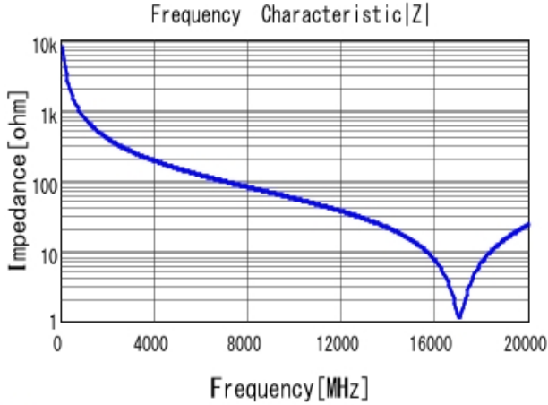
■ GRM1555C1HR20WA01 |Z| DCOV, 25degC
