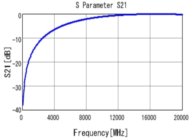
■ GRM1555C1HR20WA01 S21 DCOV, 25degC
