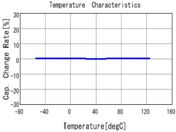
■ GRM1555C1HR20WA01 C-Temp. capchange, DCOV, AC1Vrms
