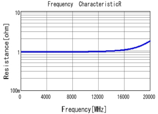
■ GRM1555C1HR20WA01 R DCOV, 25degC
