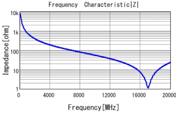
■ GRM1555C1HR20BA01 |Z| DCOV, 25degC
