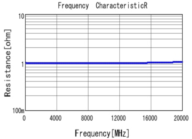
■ GRM1555C1HR10WA01 R DCOV, 25degC
