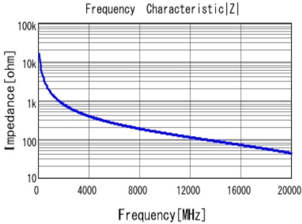
■ GRM1555C1HR10WA01 |Z| DCOV, 25degC
