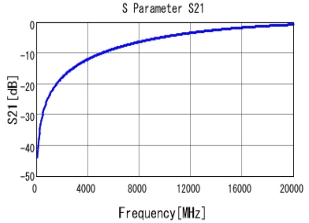
■ GRM1555C1HR10WA01 S21 DCOV, 25degC
