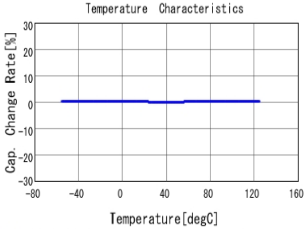
■ GRM1555C1HR10WA01 C-Temp. capchange, DCOV, AC1Vrms
