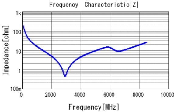
■ GRM1555C1H9R1CA01 |Z| DCOV, 25degC
