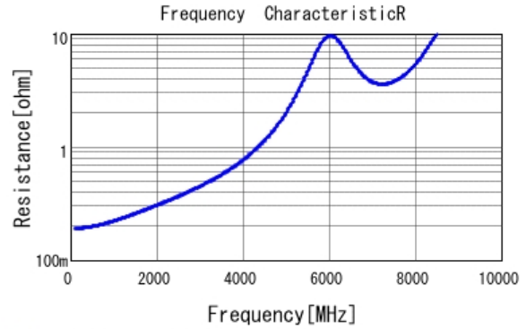
■ GRM1555C1H9R1CA01 R DCOV, 25degC
