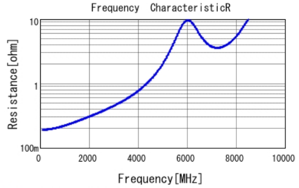
■ GRM1555C1H9R0BA01 R DCOV, 25degC
