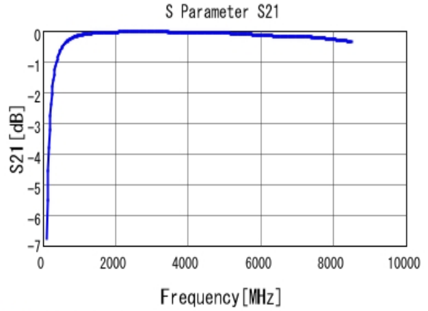
■ GRM1555C1H8R2WA01 S21 DCOV, 25degC
