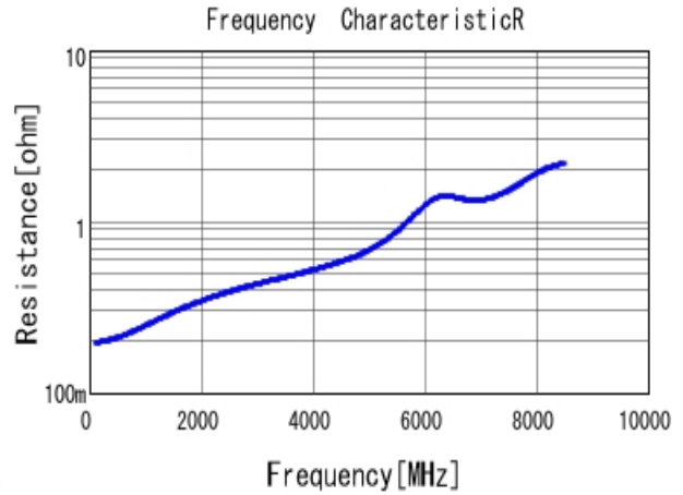
■ GRM1555C1H8R2WA01 R DCOV, 25degC
