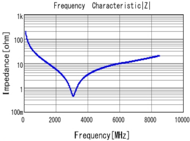
■ GRM1555C1H8R2WA01 |Z| DCOV, 25degC
