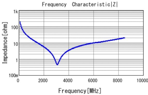
■ GRM1555C1H8R2CA01 |Z| DCOV, 25degC
