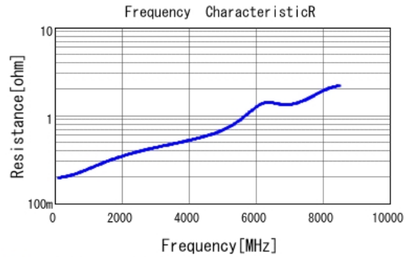
■ GRM1555C1H8R2CA01 R DCOV, 25degC
